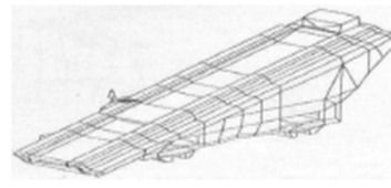
Fig. 5. Finite Element Model of Z-Slide
