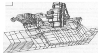
Fig.10: Finite Element Deformed Shape of Entire Machine Tool Assembly
