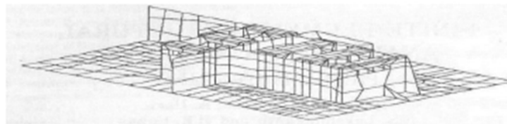
Fig. 1. Finite Element Model of Cabinet Base
