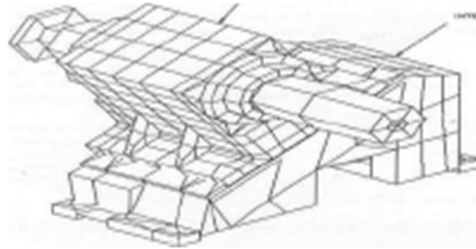
Fig8: Finite Element Model of Sub-Assembly-1 (with hidden lines removed)
