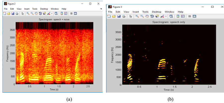
Figure 5(a) Input speech signal spectrum, (b) Output clean speech
