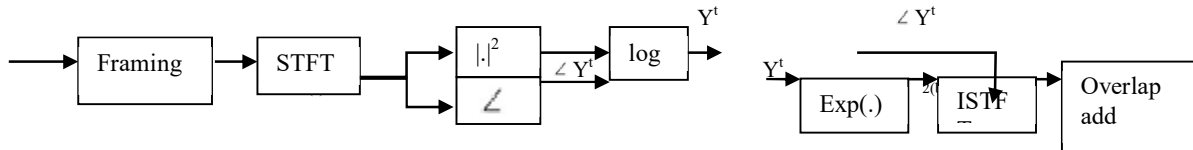
Figure 2 (a) Block of feature extraction, (b) Block of waveform reconstruction
