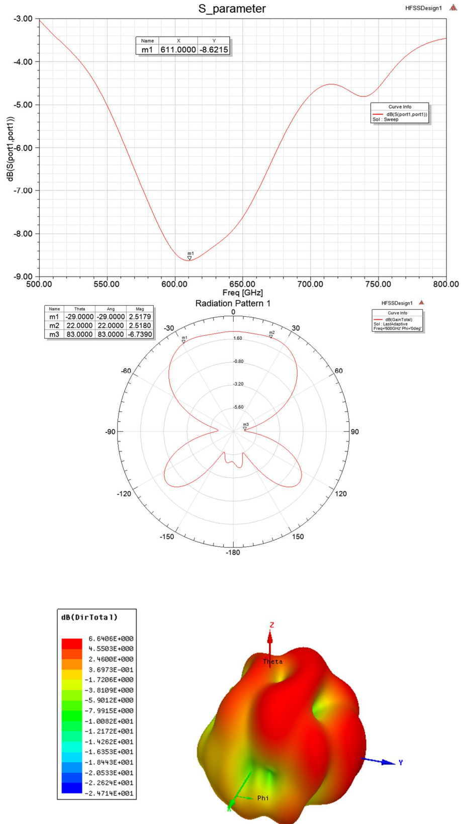
Fig. 4. (a) Return loss (b) Gain and (c) Directivity of simple microstrip patch antenna at 600GHz
