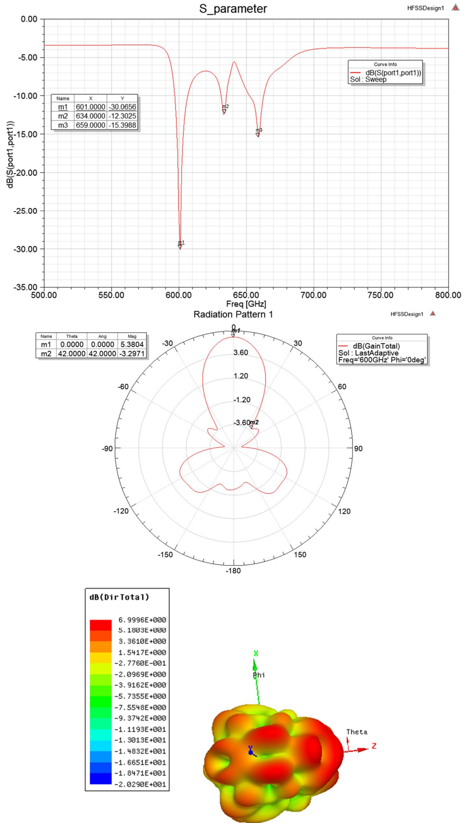
Fig. 3. (a) Return loss (b) Gain and (c) Directivity of the Proposed antenna at 600GHz
