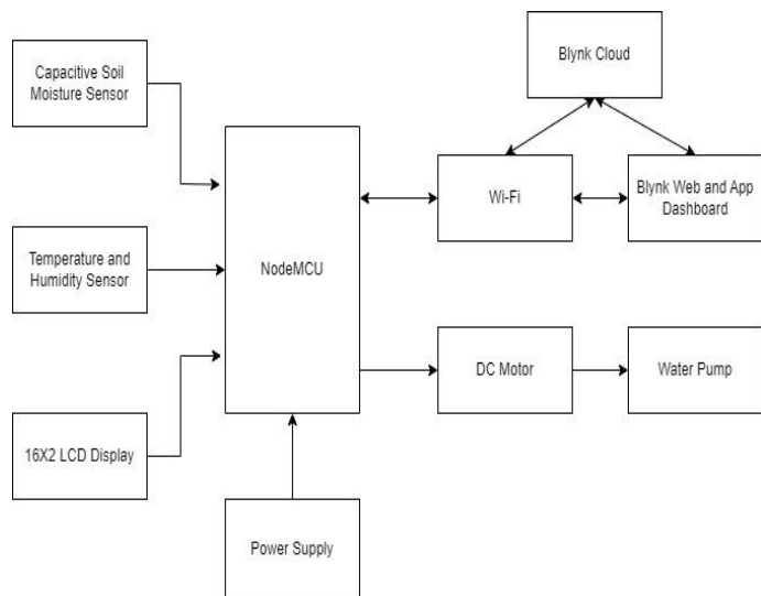
Fig. 6. Block Diagram of the proposed system
