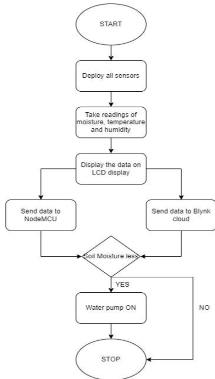
Fig. 5. Flowchart of the proposed system.
