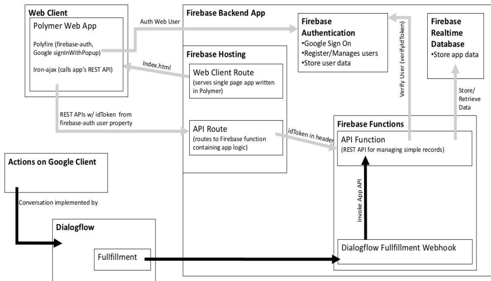
Fig.7. Firebase Flowchart for API's and Authentication.
