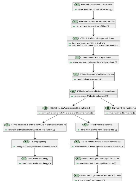
Fig.3. Full Project Workload
