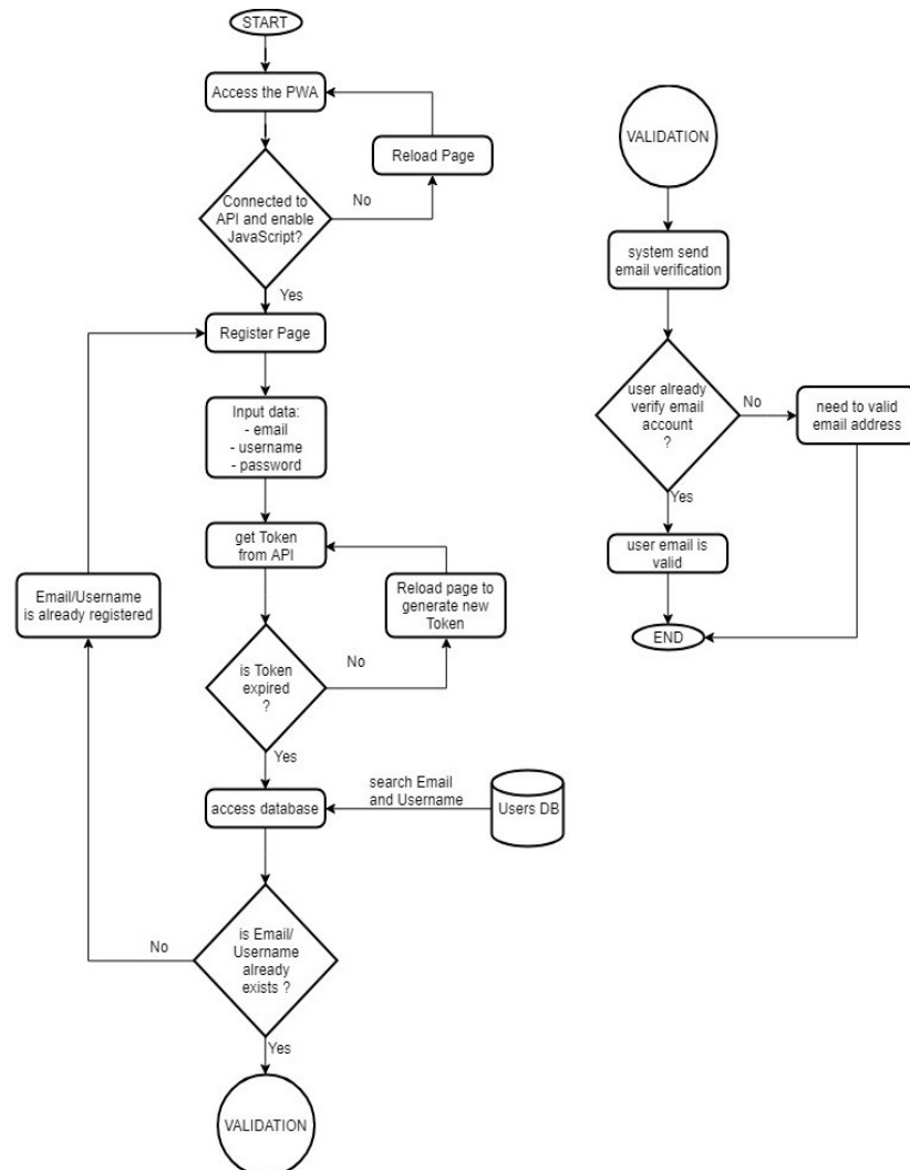
Fig.6. Flowchart for Email Validation Firebase.
