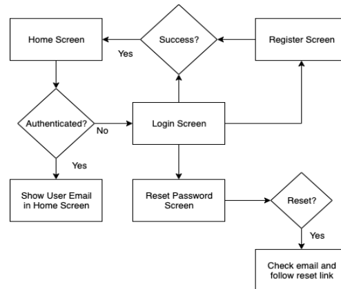
Fig.9. Login Authentication
