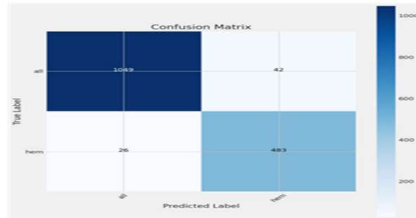
Figure 5. Representation Model - Confusion Matrix Results
