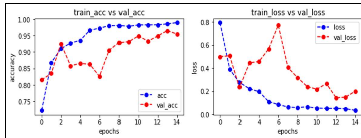
Figure 8. VGG-19 Results
