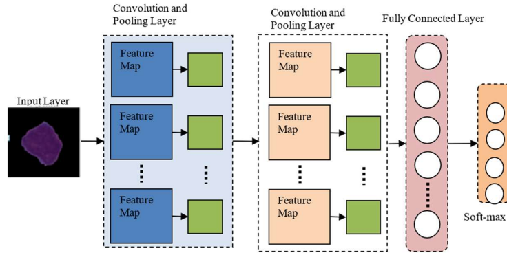
Figure 2. Architecture of leukemia disease Prediction and Classification Systems
