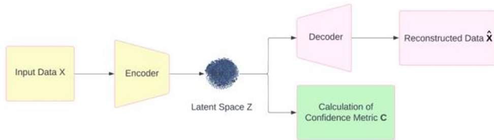
Figure 5. The main components of our VAE architecture
