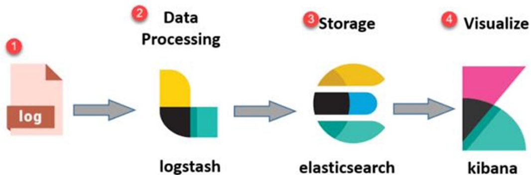
Figure 7. ELK Stack Architecture
