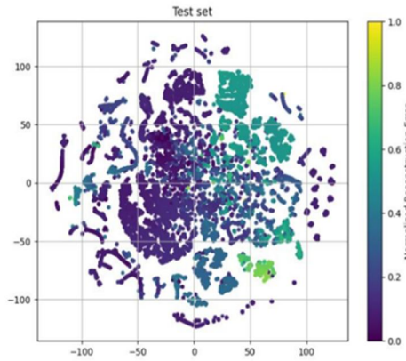
Figure 4. Visualization of Test Set
