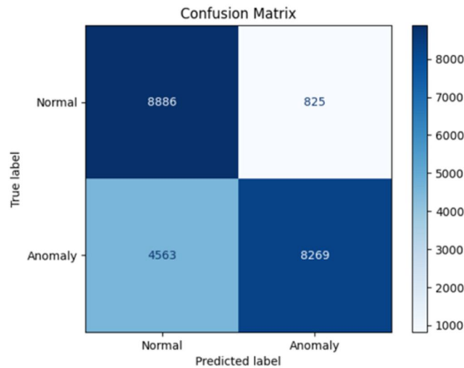
Figure 6. Confusion Matrix
