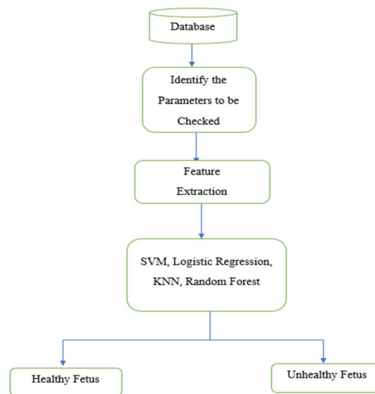
Figure 5: System Architecture
