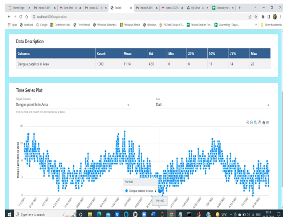
Figure 4: Times Series Various Plots
