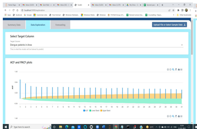
Figure 5: Target Column Selection along with ACF and PACF Plot
