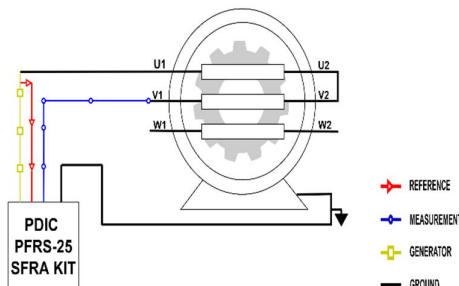
FIGURE 4. CONNECTION DIAGRAM FOR LINE MEASUREMENT
