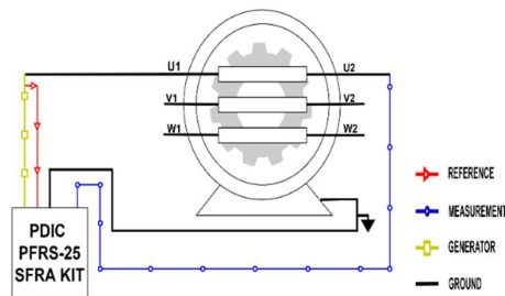
FIGURE 2 CONNECTION DIAGRAM FOR WINDING MEASUREMENT
