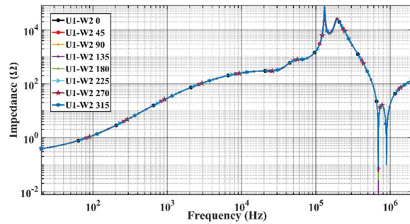
Figure 7. Frequency response for series connection
