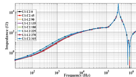
Figure 3. Frequency response for winding measurement at different positions
