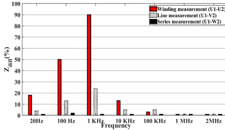
FIGURE 8. IMPEDANCE DIFFERENCE FOR THREE ARRANGEMENTS (LEFT: WINDING MEASUREMENT, MIDDLE: LINE MEASUREMENT, RIGHT: SERIES MEASUREMENT)
