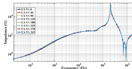
Figure 5. Frequency response for line measurement at different positions
