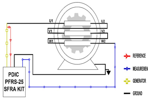
Figure 6. Connection diagram for series connection
