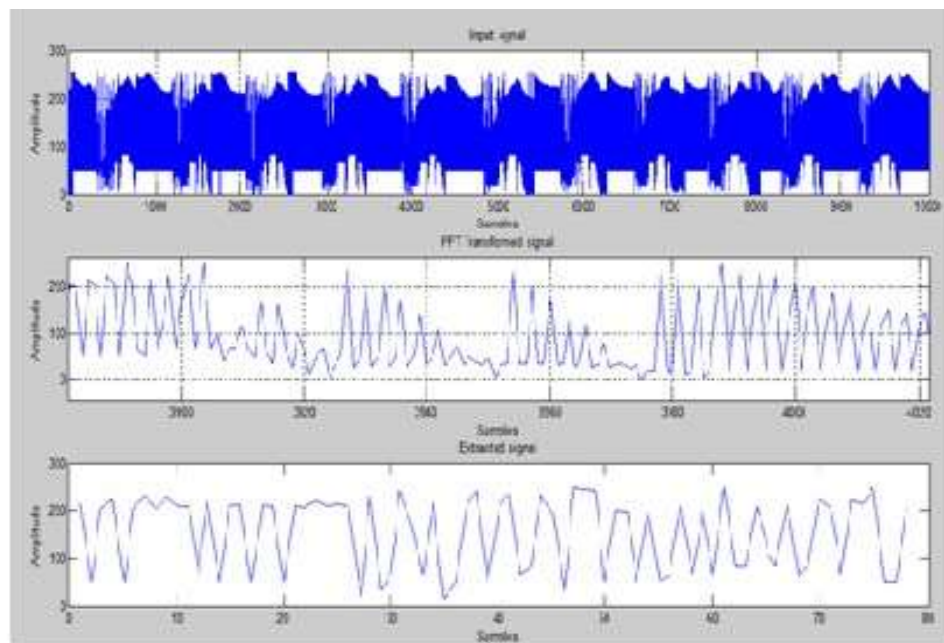
Fig.3 Transformation using for fourier Transformation
