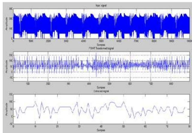
Fig.4 Transformation using Walsh-Hadamard Transformation
