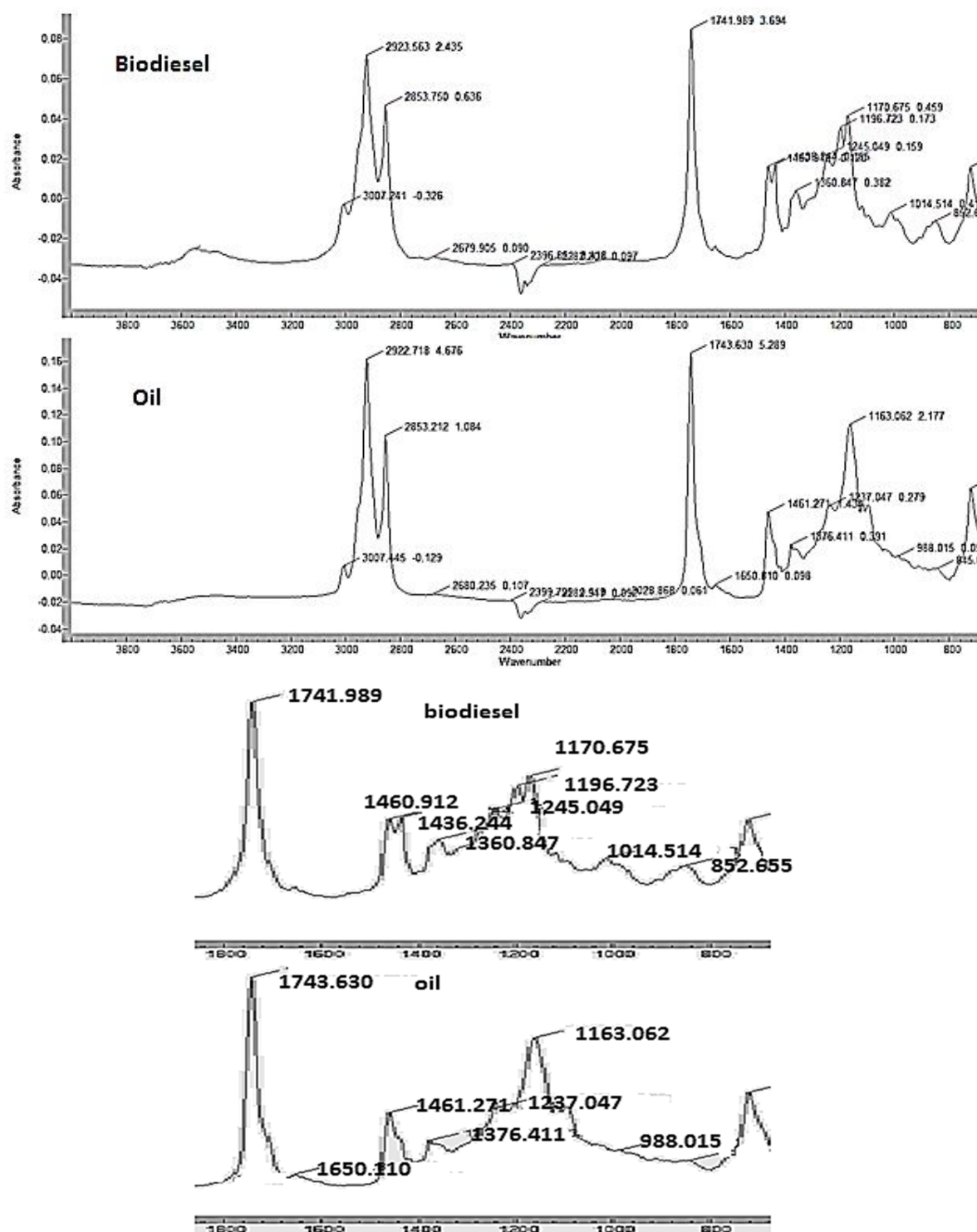
Figure 3. a) FTIR spectra of SFME and SFSO, b) Enlarged picture of region: 1800 \text{cm}^{-1} to 800 \text{cm}^{-1}
