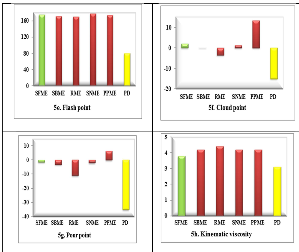
Figure 5. Comparison of fuel properties of SFME with already existing biodiesels and petrodiesel or EN14214
