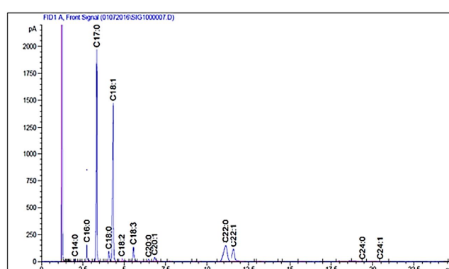
Figure 2. GC-FID of Mixture of Salvia Farinacea Methyl Ester
