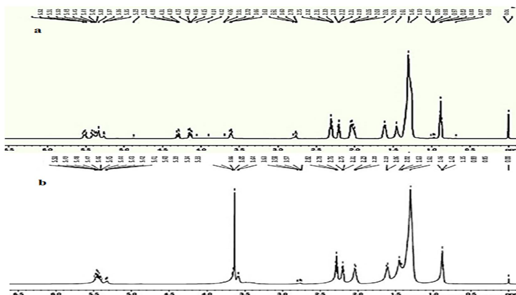
Figure 4. 1 H NMR of SFSO and SFME
