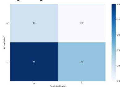
Fig.3. Confusion Matrix
