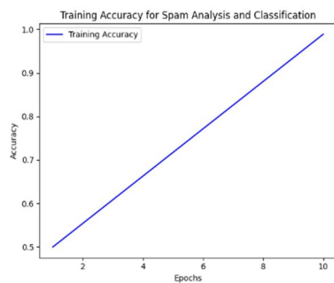
Fig.2. Accuracy graph
