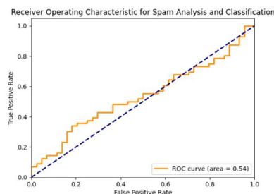
Fig.4. ROC Curve
