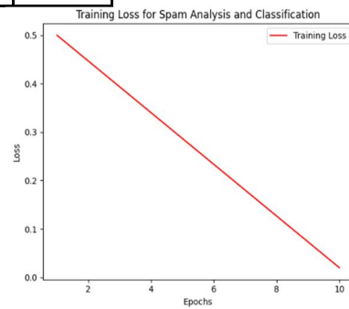
Fig.3. Loss graph
