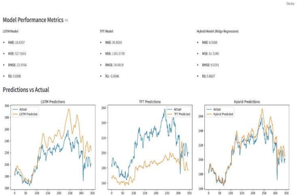
Fig 9: Model Performance Metrics
