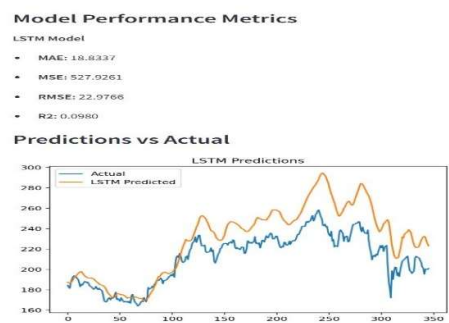
Fig 6. Model Performance
