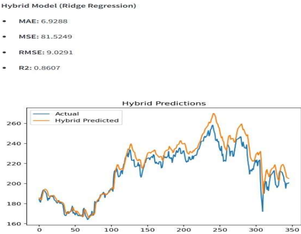
Fig 8: Hybrid Model Performance.
