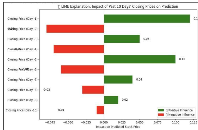
Fig 10: Feature Impact On Predicted Price.
