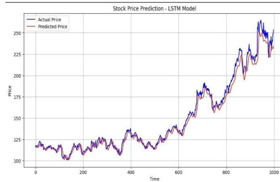
Fig 2. Actual vs Predicted Price - LSTM Model
