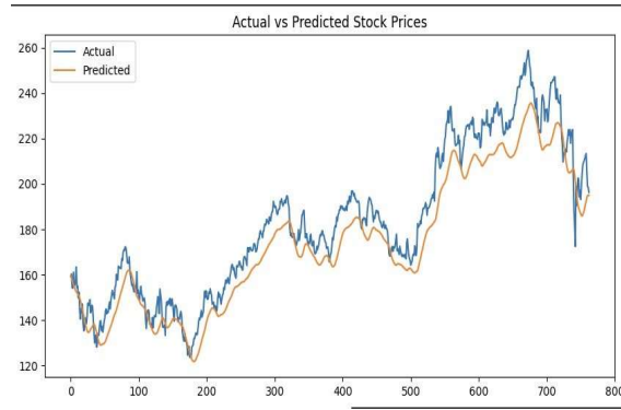
Fig 4. Actual vs Predicted Stock Price - Hybrid Model
