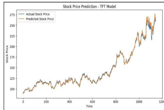
Fig 3. Actual vs Predicted Stock Price - TFT Model
