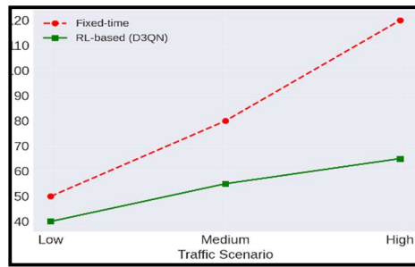
Figure 2. Average Vehicle Delay
