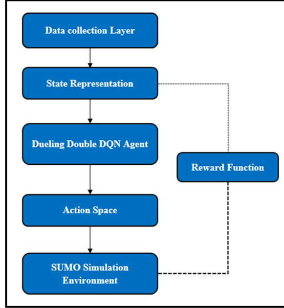
Figure 1. System Architecture of Adaptive Traffic Signal Control using Dueling Double Deep Q-Networks (D3QN).
