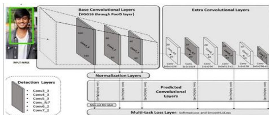
Figure 2. Architecture of Single Shot Scale-invariant Face Detector (S3FD)
