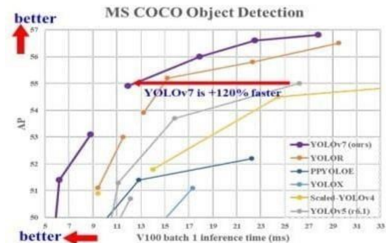
Figure 1 .Comparisons between different yolo models
