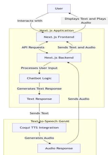
Fig. 2. Architecture. Figure 2 Shows A Graphic Representation Of The Proposed Architecture
