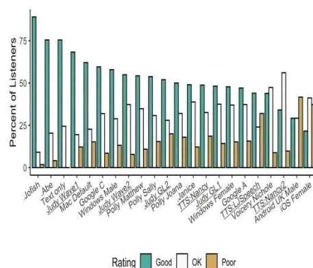
Fig. 2.2.2 TTS Performance [47]
