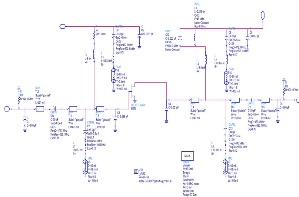
Figure2. Circuit diagram for LNA with HEMT
