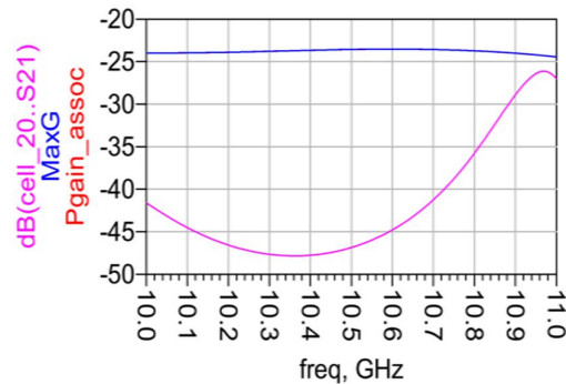
Figure 3. Gain & Insertion loss
