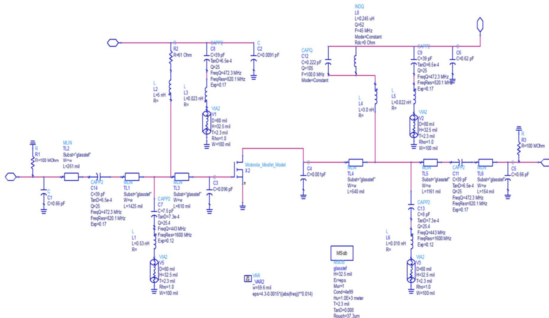
Figure5. Circuit diagram for LNA using MOSFET
