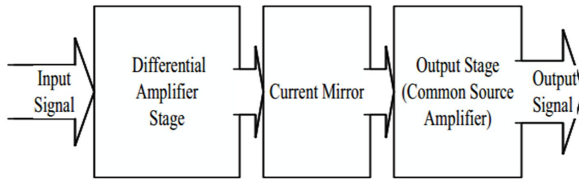
Figure1. Block diagram of LNA
