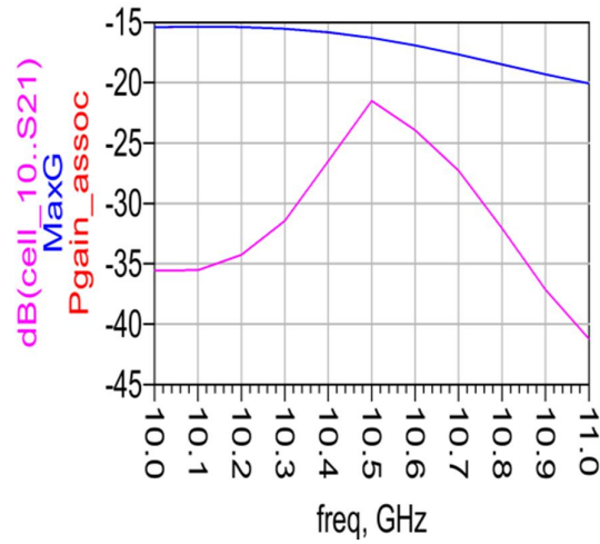
Figure 6. Gain & Insertion loss
