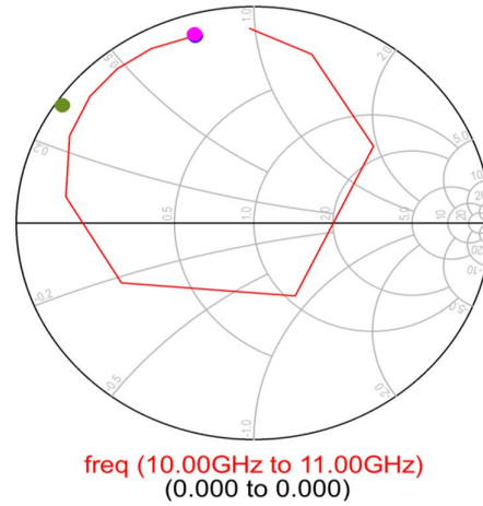
Figure 7. VSWR
