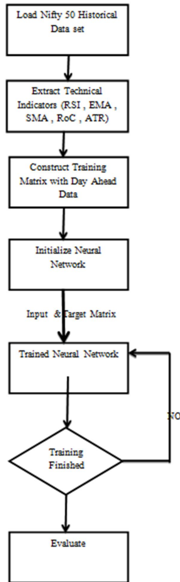
Fig 1 Proposed Methodology
