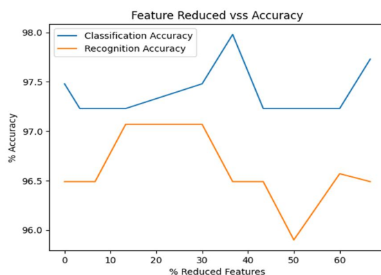
Figure 3. Effect of feature reduction on accuracy
