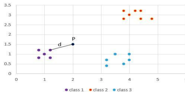
Figure 3. Scatter Plot of 2D patterns and working of KNN
