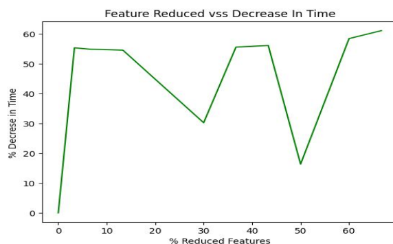
Figure 2. Plot of percentage reduction in features versus percentage reduction in time.
