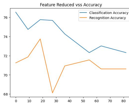
Figure 4. Effect of feature reduction on accuracy
