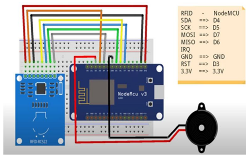
Fig. 1 : Circuit diagram of RFID based attendance monitor system
