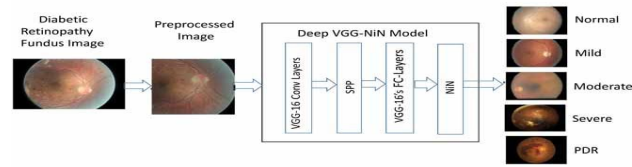
Figure 4: Deep VGG-NiN model for the classification of Diabetic Retinopathy Stages using Fundus Images.
