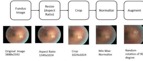
Figure 2 : Preprocessing steps.
