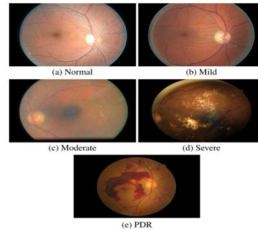
Figure 1 : The different stages of DR
