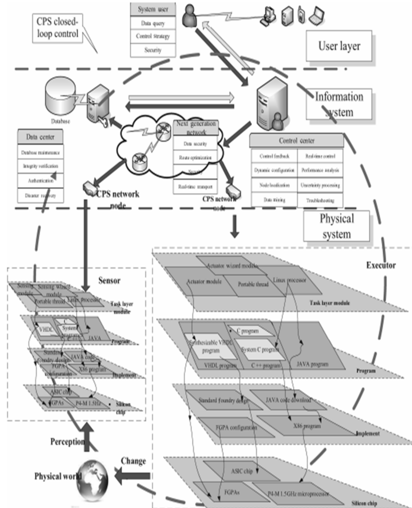
Figure 1 Architecture of Cyber Physical Systems [1]
