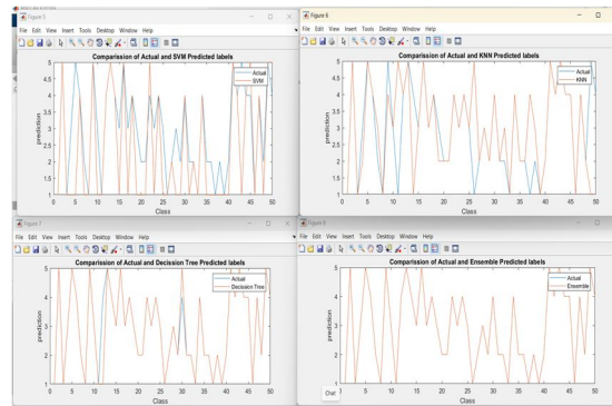
Fig 5.9: Different classifiers with comparison of actual and prediction data
