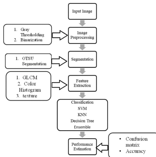
Fig 3.1: Block diagram for fruit classification using multiple classifiers
