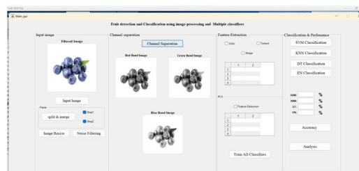
Fig 5.2: Input image, preprocessing and Channel Suppuration with RGB components
