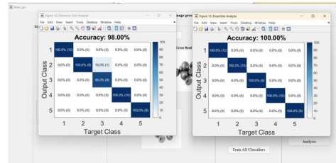
Fig 5.8: Confusion matrix for 50 fruit random data inputs for analysis DT, Ensemble
