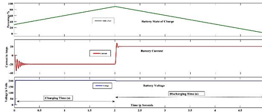
Figure 15: Battery Charging & Discharging Cycle, 0-2s=Charging & 3-5s=Discharging
