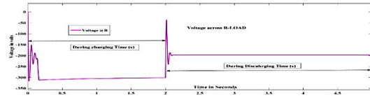
Figure 9: Output Voltage across R-Load during charging=300 V & discharging=200 V Figure 10: Boost Operated Output Voltage, 300 V
