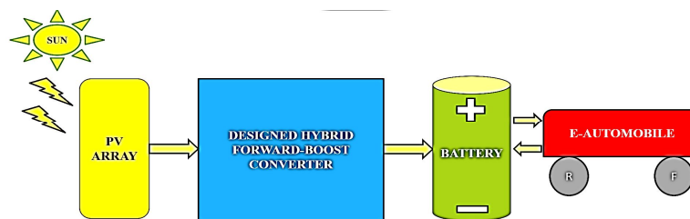
Figure 1: Block Diagram
