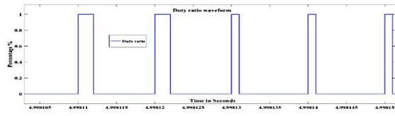
Figure 7: PID Generated Duty ratio during charging
