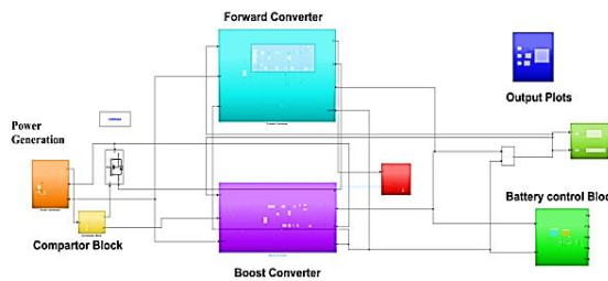
Figure 3: Forward-Boost Hybrid Converter
