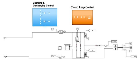
Figure 4: Battery Control Block
