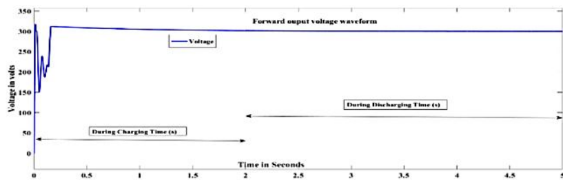
Figure 5: Forward Operated Output Voltage, 300V
