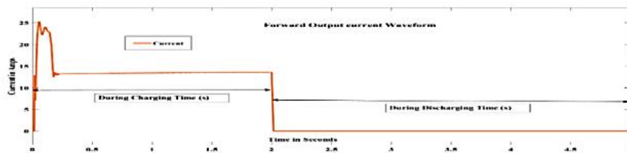
Figure 1: Forward Operated Output Current, I_{avg} =15-20A, 0-2s=Charging & 3-5s=Discharging
