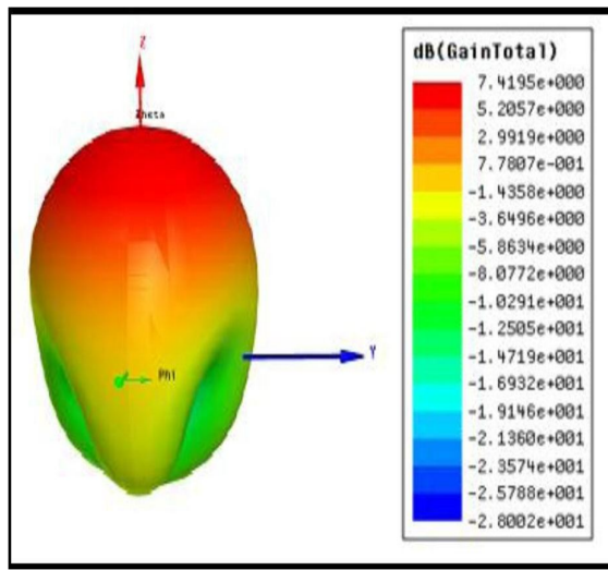
Figure 6: 3D polar plot of Gain
