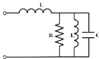
Figure 1: Microstrip line probe
