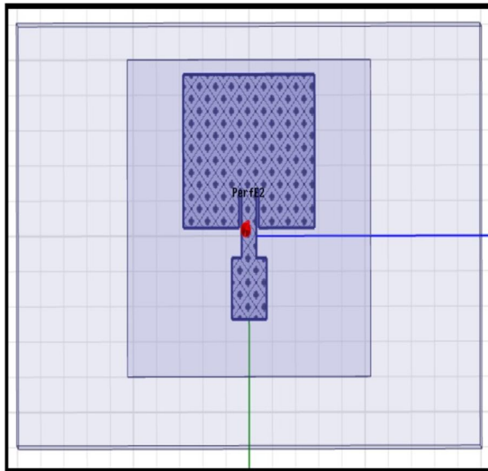
Figure 5: Design of rectangular microstrip patch antenna with inset fed in HFSS software
