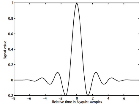
Figure 7 Sinc reference function, windowed with a raised cosine window.
