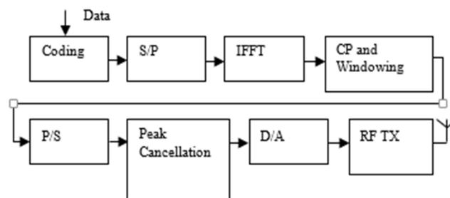
Figure 8 OFDM transmitter with peak cancellation.
