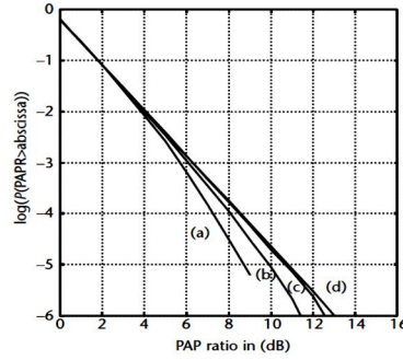
Fig 1. PAP distribution of an OFDM signal with (a) 12, (b) 24, (c) 48, and (d) an infinite number of SCs (pure Gaussian noise). Four times oversampling used in simulation; total number of simulated samples is 12 million.
