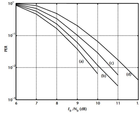
Figure 6 PER versus E_b/N_0 for 64-byte packets in AWGN. OFDM signal is clipped to a PAP ratio of (a) 16 (no distortion), (b) 6, (c) 5, and (d) 4 dB.
