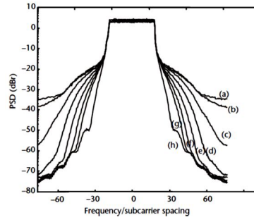
Figure 5 Frequency spectrum of an OFDM signal with 32 SCs with peak windowing at a threshold level of 3 dB above the RMS amplitude. Symbol length is 128 samples (4 times oversampled) and window length is (a) 3, (b) 5, (c) 7, (d) 9, (e) 11, (f) 13, and (g) 15 samples. Curve (h) represents the ideal OFDM spectrum.
