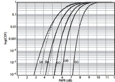
Figure 3 CDF of the PAP ratio (PAPR) for a number of SCs of (a) 32, (b) 64, (c) 128, (d) 256, and (e) 1,024. Solid lines are calculated; dotted lines are simulated.
