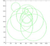
Fig 20: Output image
