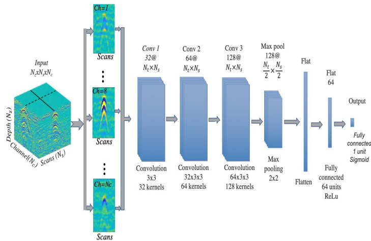
Fig 2. CNN Architecture
