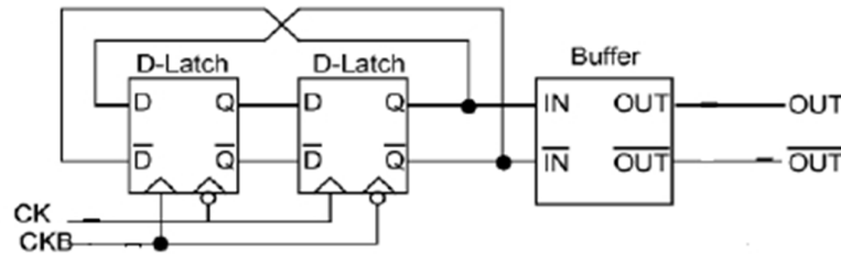
Figure 2 frequency divider
