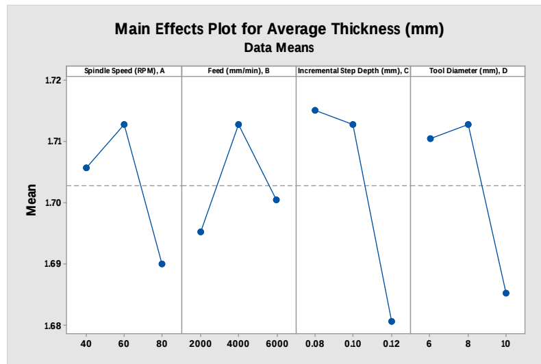
Figure 10. Main effect plot for Average Thickness
