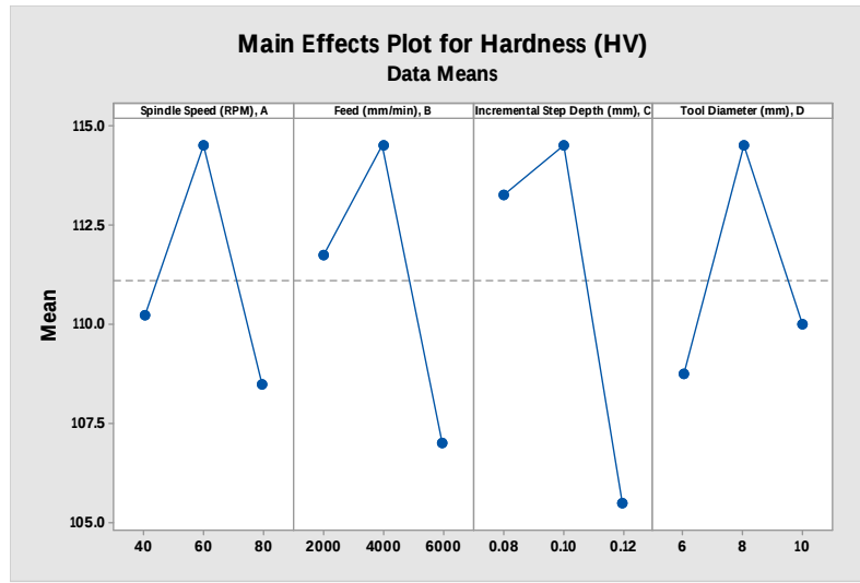
Figure 11. Main effect plot for Hardness
