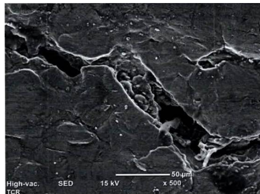
Figure 15. SEM image of Specimen No. 4 at X500
