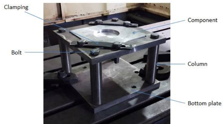
Figure 2. DM Stretching Model Setup
