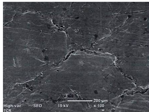
Figure 12. SEM image of Specimen No. 1 at X100
