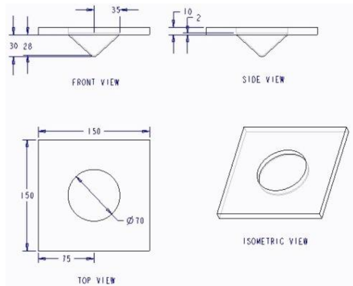
Figure 1.Component's drawing
