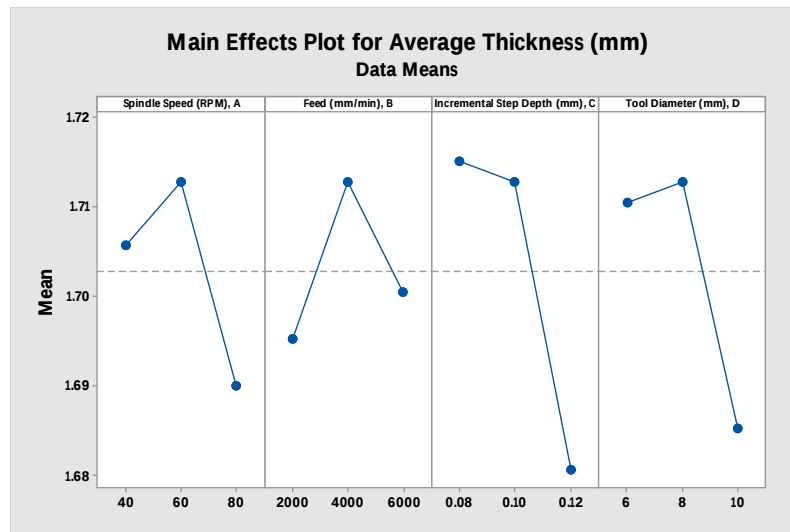
Figure 9 Main effect plot for factors A,B,C, and D
