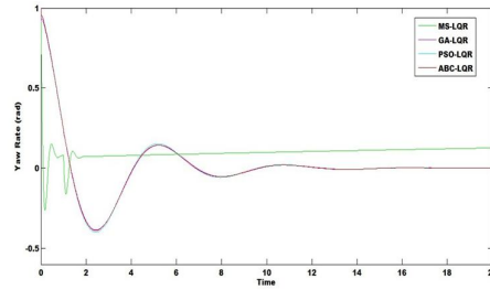
Fig. 5. Yaw Rate Deviation for Case (iii)
