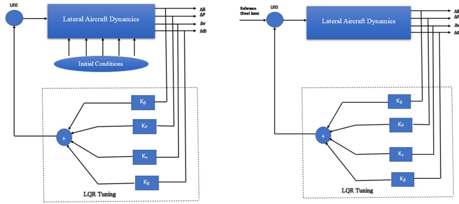
Fig. 2. Aircraft System with Initial Conditions and Reference Inputs
