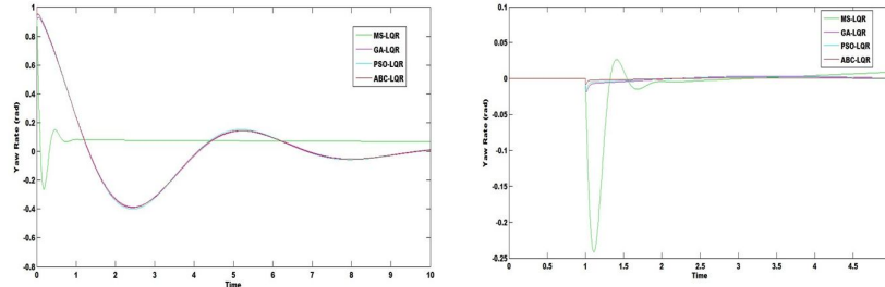
Fig. 4. Yaw Rate Deviation for Case (i) and Case (ii)
