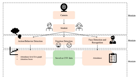
Fig. 6. Activity Diagram
