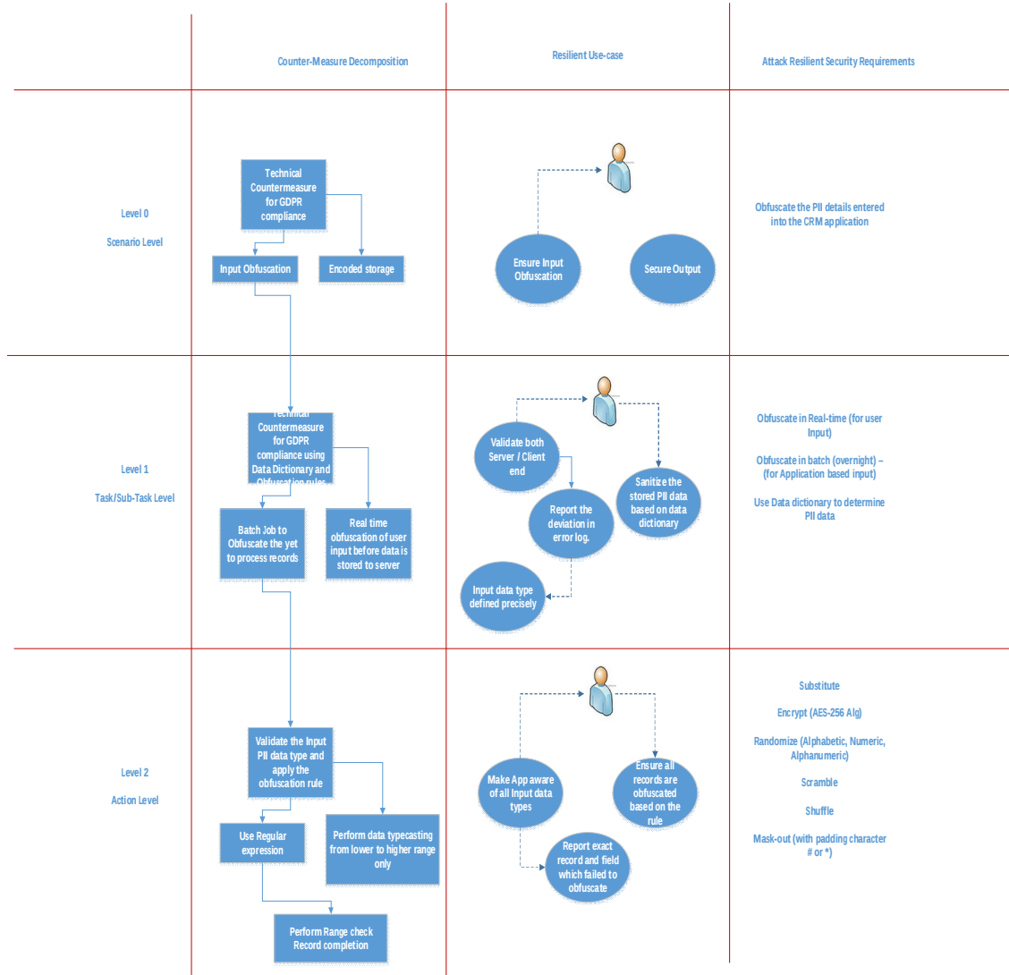
Fig 2 – Mapping of requirements to possible threats and equivalent countermeasures
