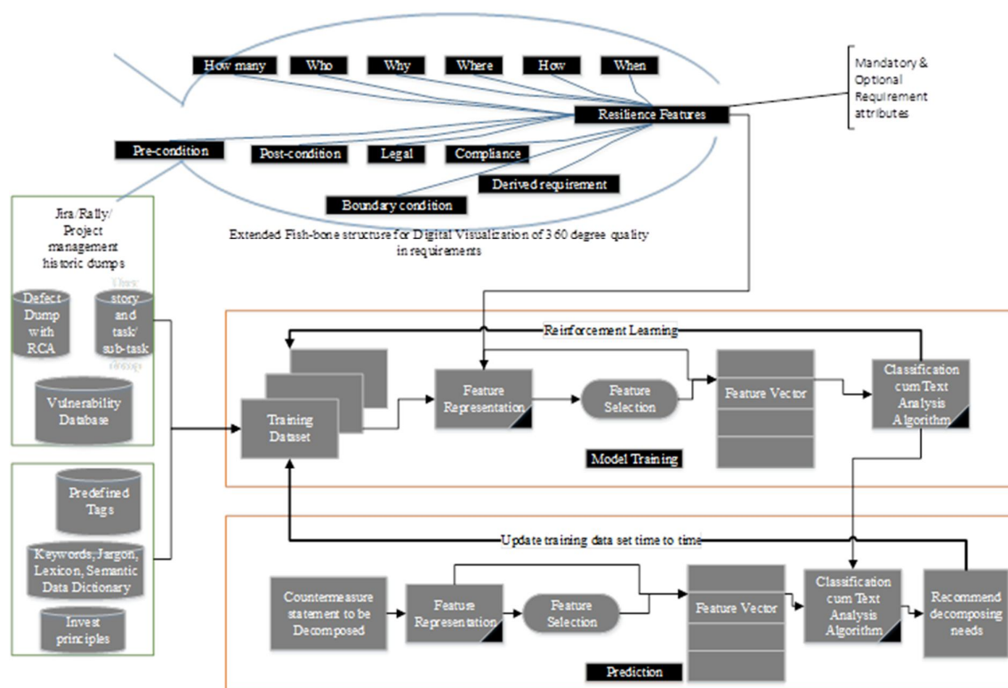
Fig 3 – Extended fish bone with reinforcement machine learning
