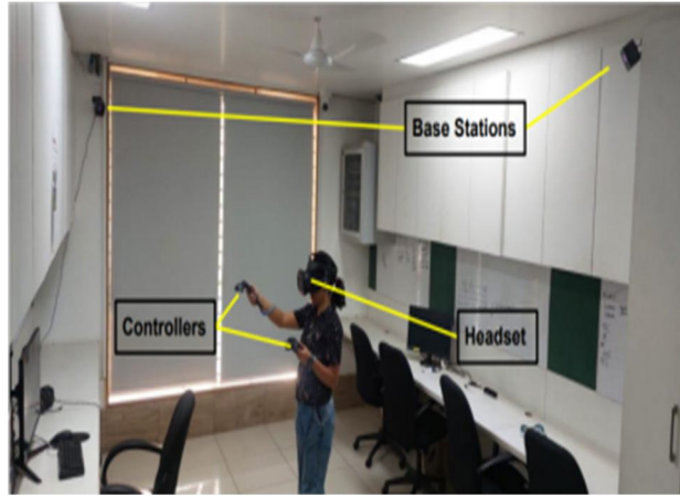
Figure 3. The VR setup that was established for this project
