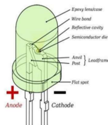
Fig -5 Light Emitting Diode
