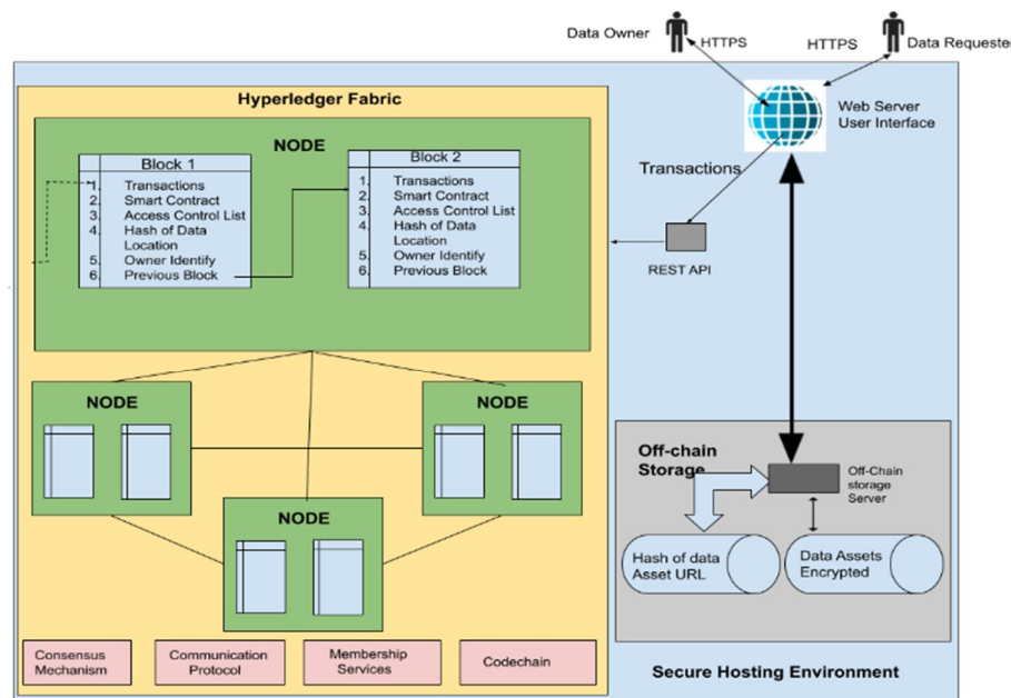
Fig. 1: Architecture
